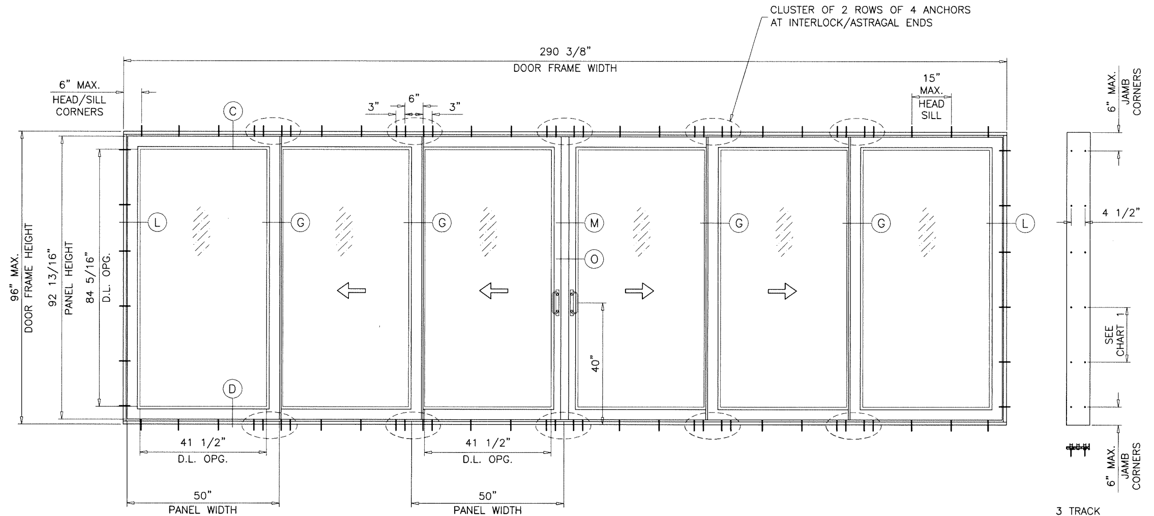
TYPICAL ELEVATION
